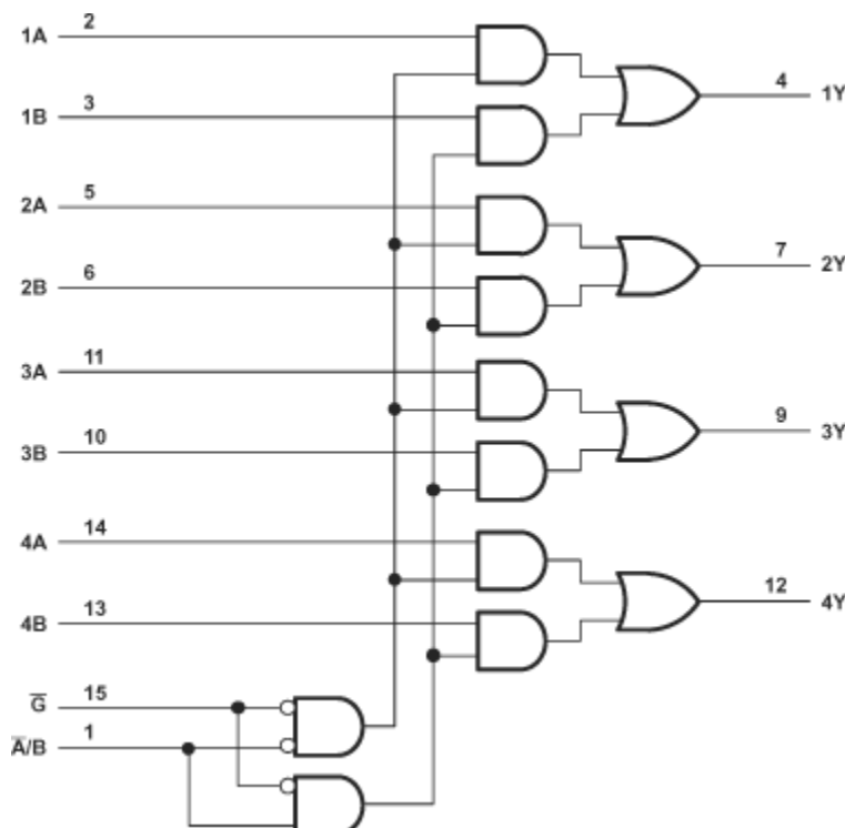
Figure 7-1. Logic Diagram (Positive Logic)
