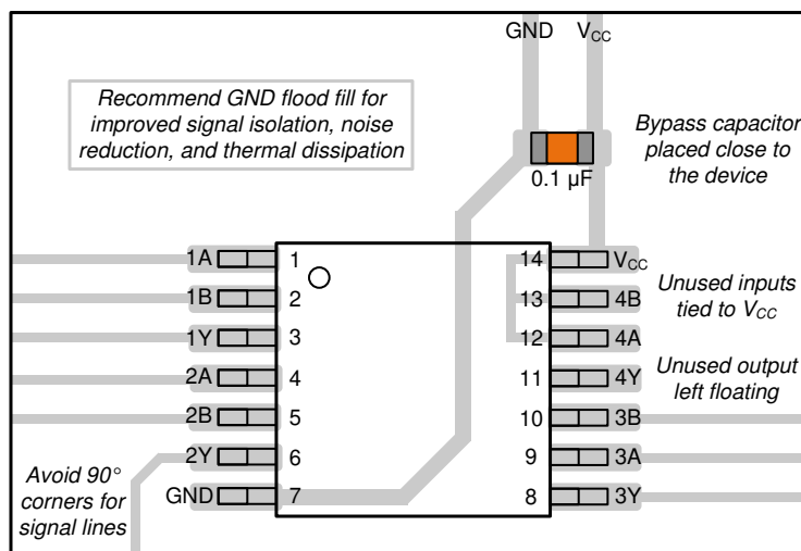
Figure 12-1. Example Layout for the SN74LV4T08-Q1
