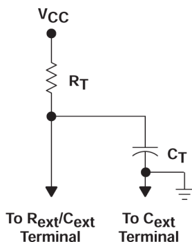
Figure 7-1. Timing-Component Connections
