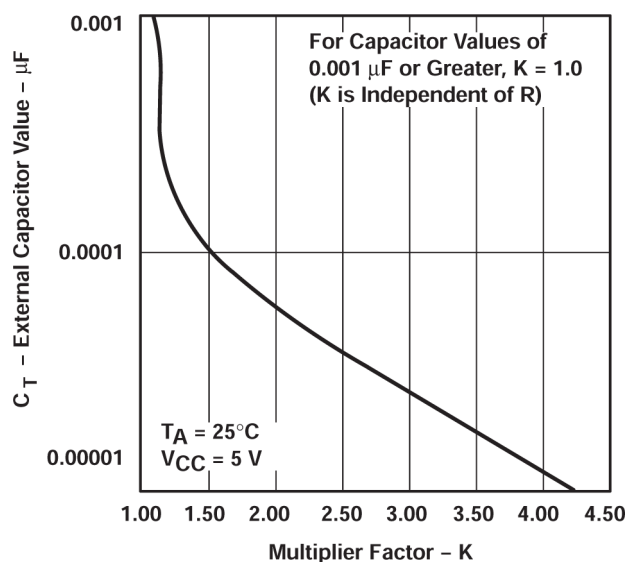
Figure 7-5. External Capacitance vs Multiplier Factor
