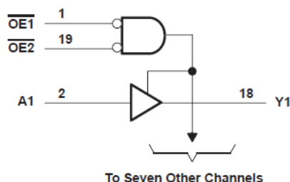
Functional Block Diagram
