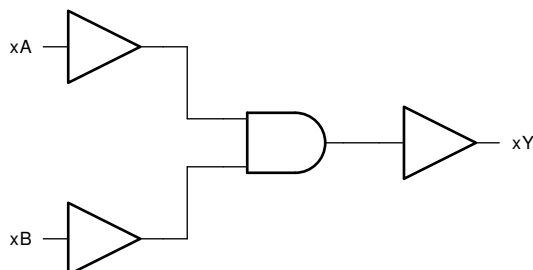
Figure 6-1. Functional Block Diagram
