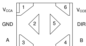
Figure 4-5. DTQ Package 6-Pin X2SON (Transparent Top View)
