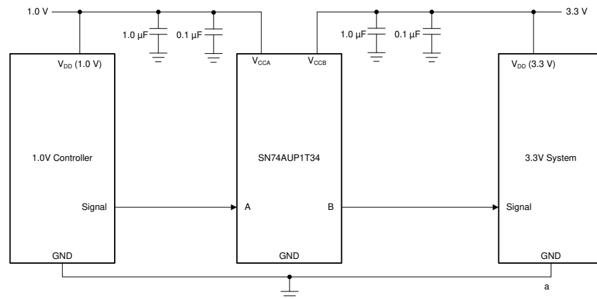
Figure 4. Typical Application Example
