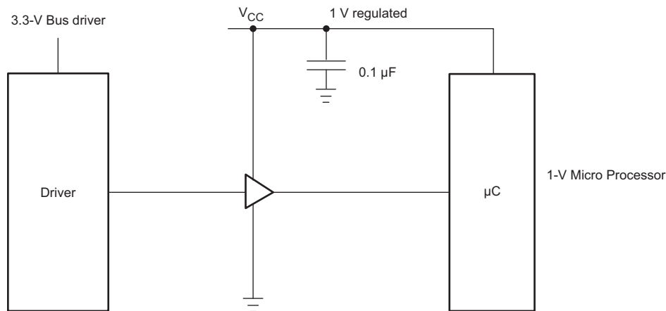
Figure 5. Typical Application
