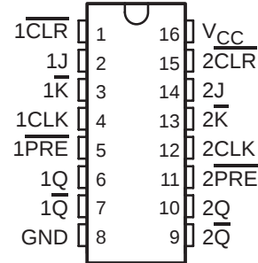
SN54ALS109A, SN54AS109A ... J PACKAGE SN74ALS109A, SN74AS109A ... D OR N PACKAGE (TOP VIEW)
