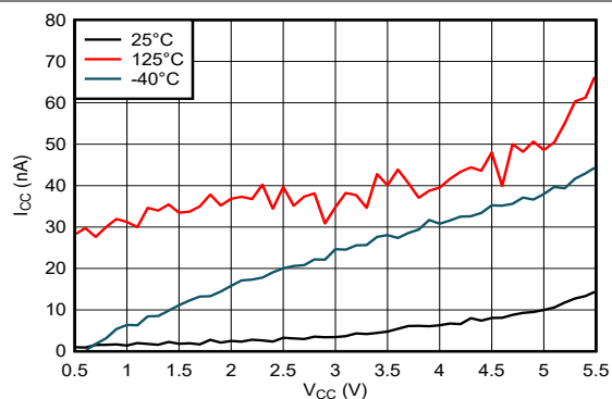
Figure 5-2. Supply Current Across Supply Voltage
