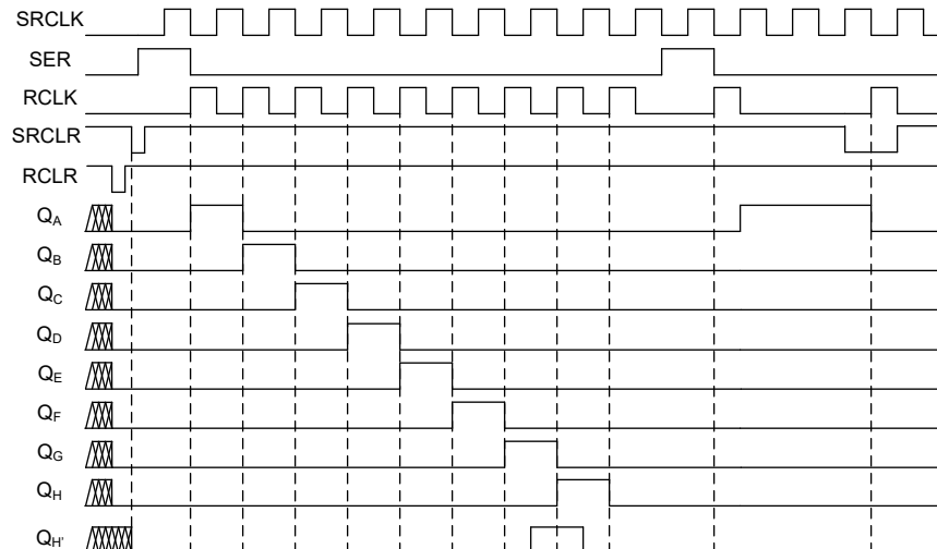
Figure 5-1. Timing Diagram
