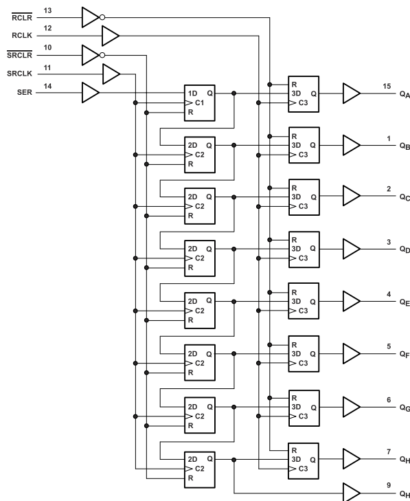
Simplified Schematic
