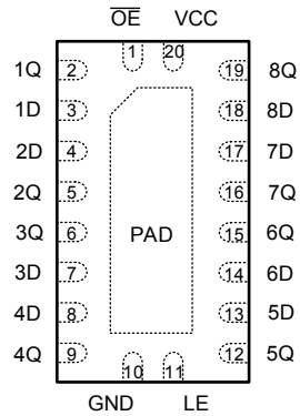
Figure 4-1. SN74AHCT373-Q1 RKS Package (Top View)
