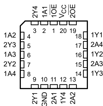
Figure 4-2. SN54AHC244 FK Package, 20-Pin LCCC (Top View)
