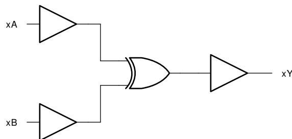
Logic Diagram
