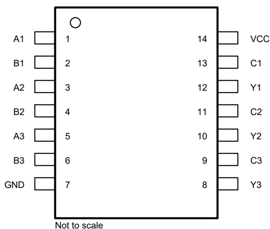
Figure 4-1. SN74ACT3G98-Q1 PW Package, 14-Pin TSSOP (Top View)
