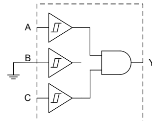
2-Input AND Gate
