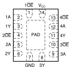
Figure 4-1. SN74ACT125 BQA Package (Top View)
