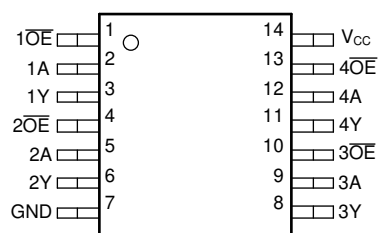
Figure 4-2. SN74ACT125, PW Package (Top View)
