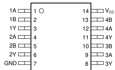
Figure 4-2. SN74AC132-Q1, PW Package (Top View)
