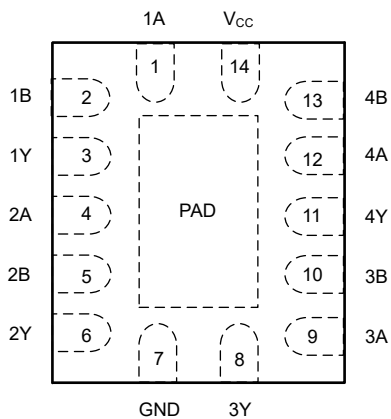
Figure 4-1. SN74AC132-Q1 BQA Package (Top View)
