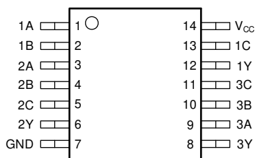
Figure 4-1. SN74AC10-Q1 PW Package (Top View)
