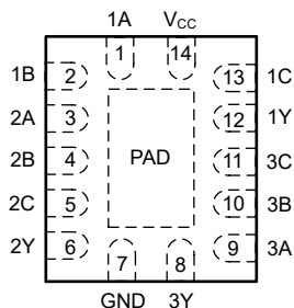
Figure 4-2. SN74AC10-Q1 BQA Package (Top View)
