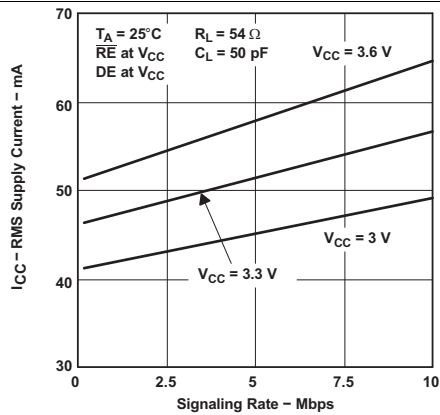
Figure 3. RMS Supply Current vs Signaling Rate
