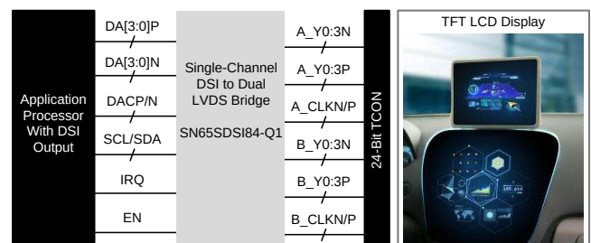
Figure 1. Typical Application
