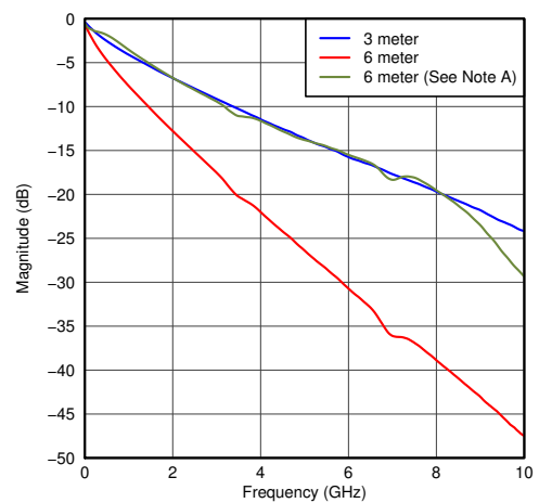
Figure 9-4. Cable Mode – Frequency Domain
