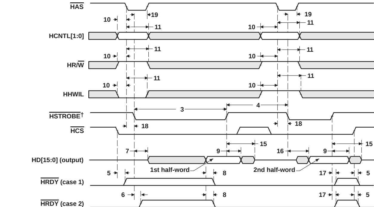
Figure 28. HPI Read Timing ( \overline{\text{HAS}} Used)
