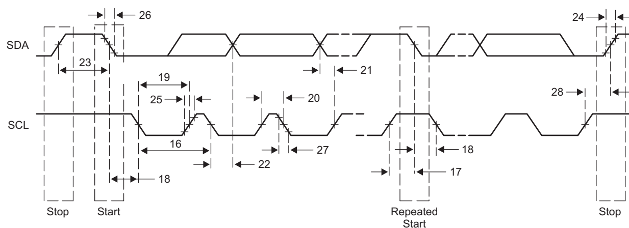
Figure 7-41 I 2 C Transmit Timings
