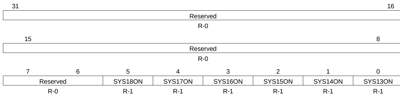
Figure 7-32. SYSCLOCK Status Register (SYSTAT)
