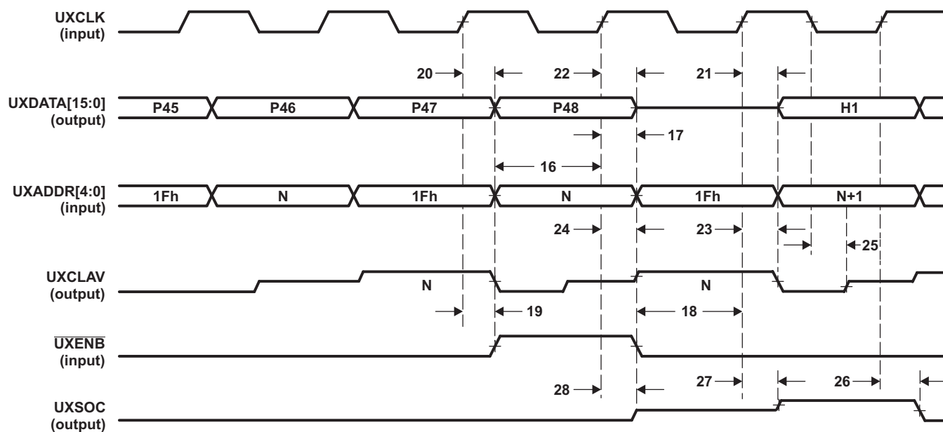
Figure 7-64. UTOPIA Slave Transmit
