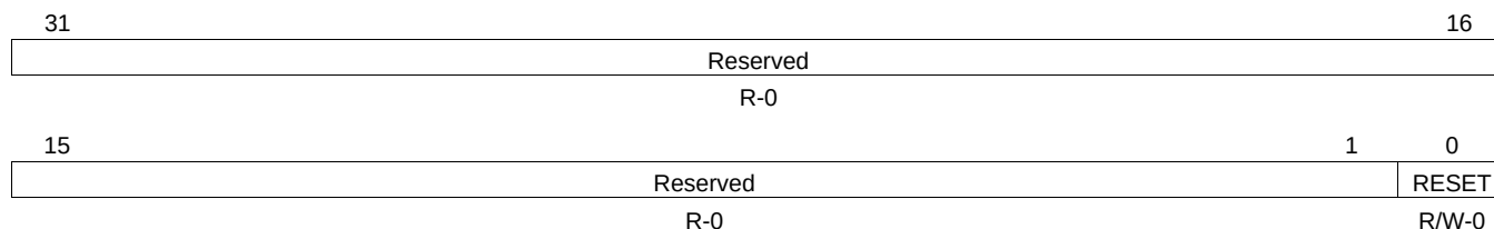
Figure 3-4. RMII Reset Registers (RMIIRESET0 and RMIIRESET1)
