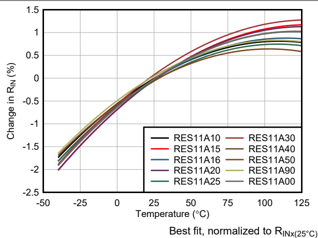
Figure 5-7. R_{INX} vs Temperature
