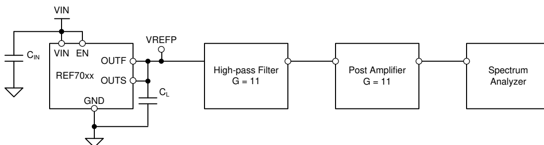
Figure 8-12. Broadband Noise Test Setup
