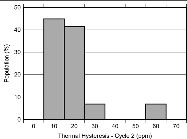
Figure 7-8. Thermal Hysteresis Distribution –40°C to 85°C, Cycle 2
