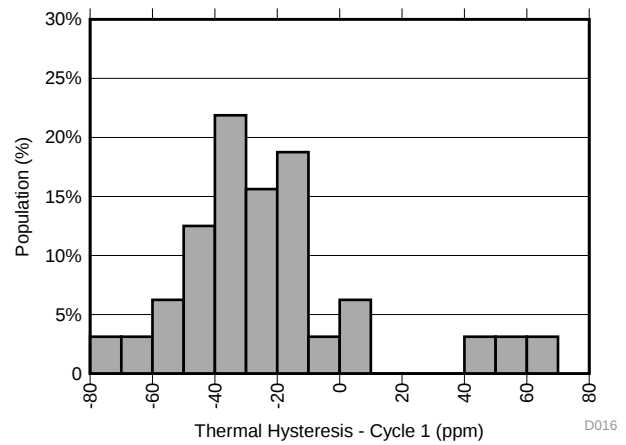
Figure 14. Thermal Hysteresis Distribution (Cycle 1)
