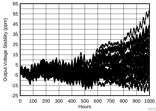
Figure 24. Long Term Stability - 1000 hours ( V_{REF} )
