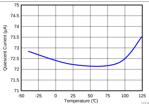
Figure 1. Temperature Drift
