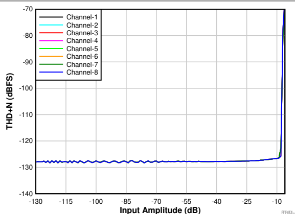
Figure 5-5. THD+N vs Input Amplitude
