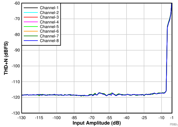
Figure 5-9. THD+N vs Input Amplitude
