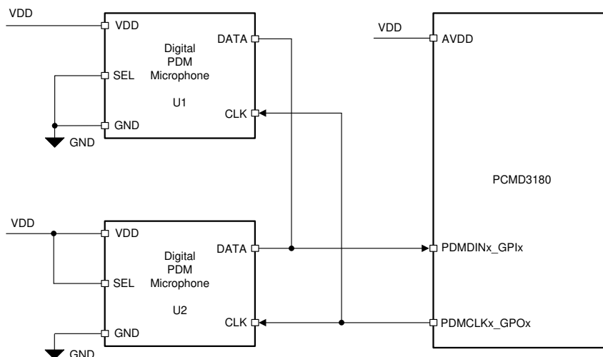
Figure 6-14. Digital PDM Microphones Connection Diagram to the PCMD3180-Q1
