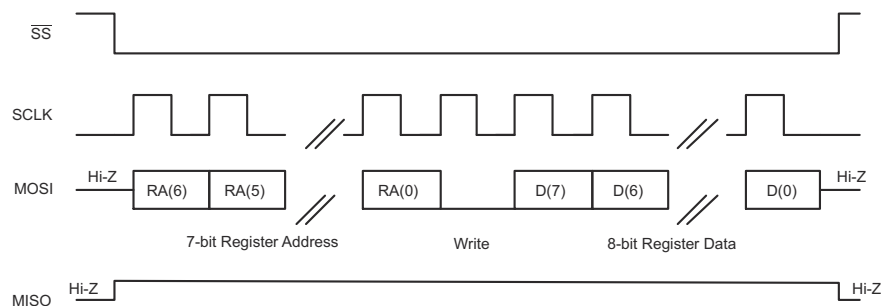
Figure 6-68. SPI Single-Byte Write Transfer
