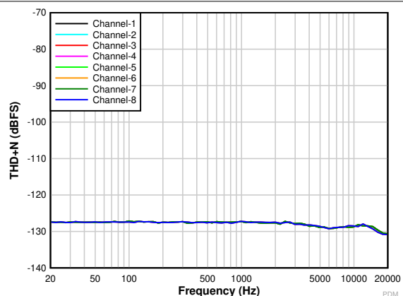
Figure 5-6. THD+N vs Input Frequency With a -20-dBr Input
