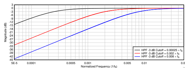
Figure 6-17. HPF Filter Frequency Response Plot
