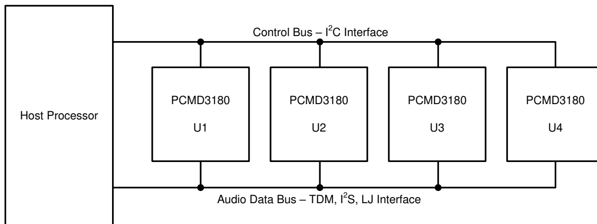
Figure 6-13. Multiple PCMD3180-Q1 Devices With Shared Control and Audio Data Buses
