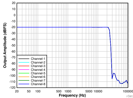
Figure 5-11. Frequency Response With a –20-dBr Input
