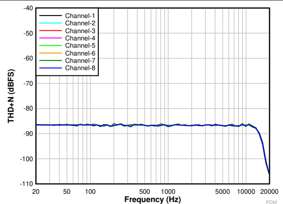
Figure 5-14. THD+N vs Input Frequency With a – 20-dBr Input
