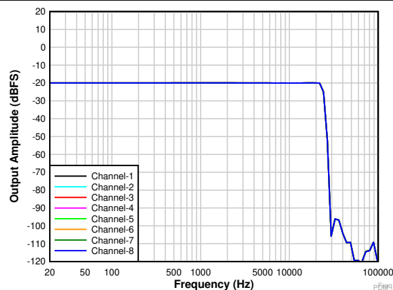
Figure 5-7. Frequency Response With a -20-dBr Input
