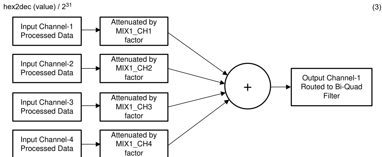
Figure 6-18. Programmable Digital Mixer Block Diagram
