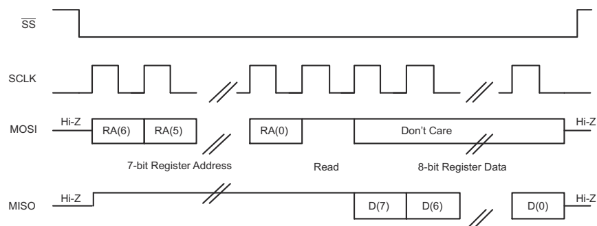
Figure 6-69. SPI Single-Byte Read Transfer
