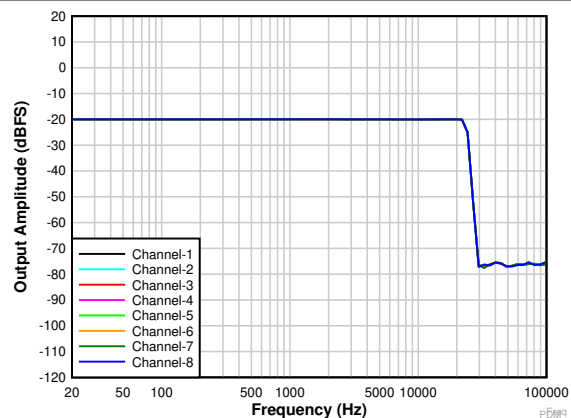
Figure 5-15. Frequency Response With a -20-dBr Input
