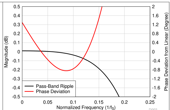
Figure 6-62. Ultra-Low-Latency Decimation Filter Pass-Band Ripple and Phase Deviation
