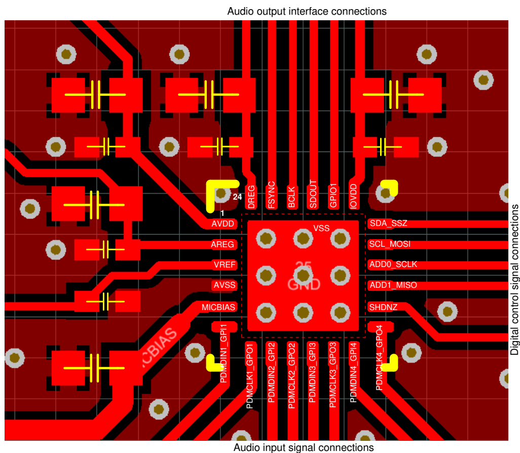
Figure 10-1. Layout Example
