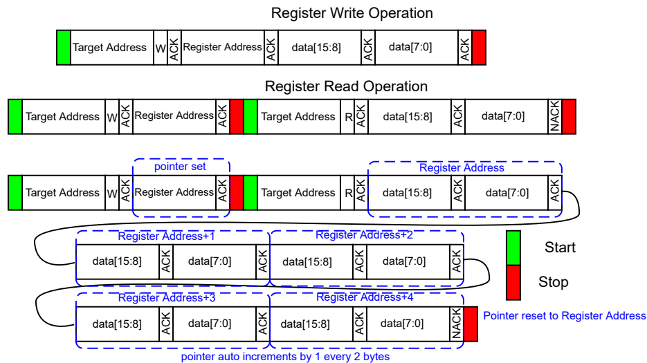
Figure 6-7. I 2 C Operations
