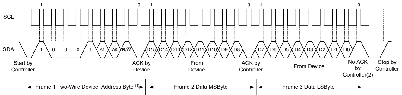
Figure 6-6. I 2 C Read Example
