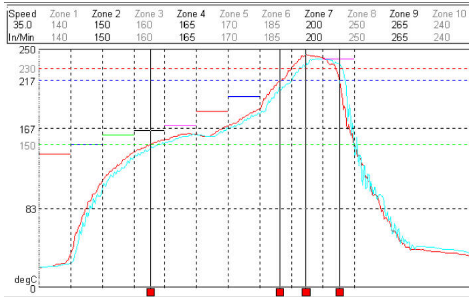
Figure 8-11. Recommended Solder Reflow Temperature Profile
