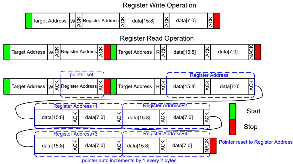
Figure 6-8. I²C Operations
