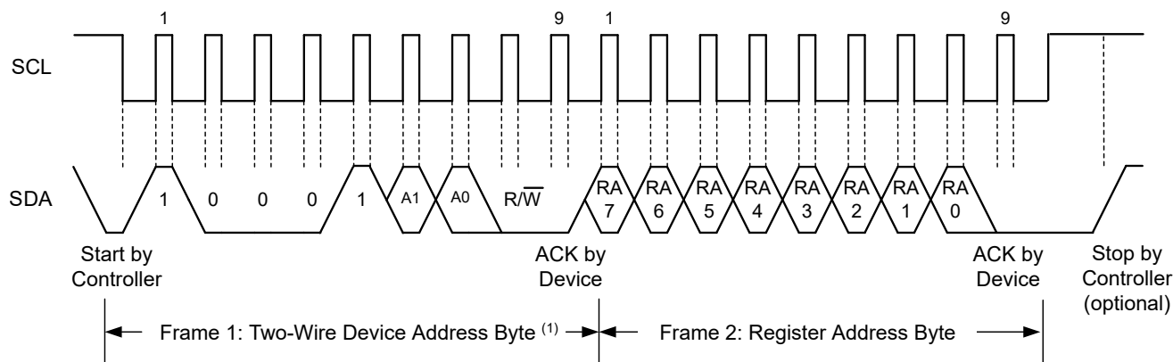
Figure 6-5. Setting the I²C Register Address
