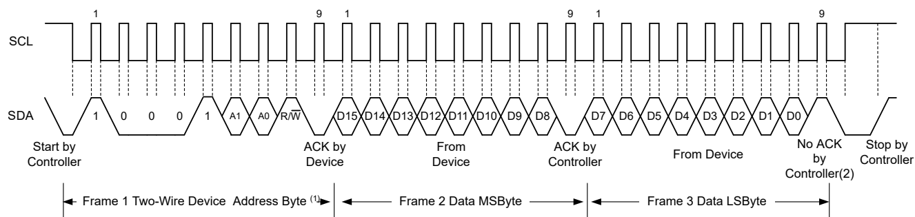
Figure 6-7. I²C Read Example
