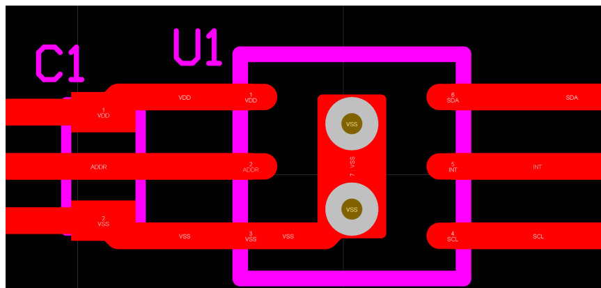
Figure 8-12. Layout Example for DNP Package
