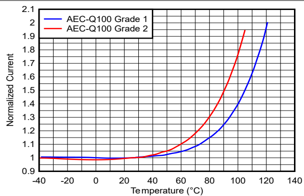
Figure 5-14. Standby Current vs Temperature
