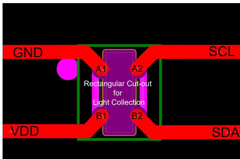
Figure 8-14. Layout Example for YMN Package With Rectangular Cut Out
