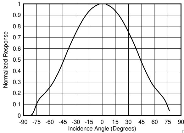
Figure 8-7. Angular Response of this FPCB Design Along the Less-Restricted Rotational Axis
