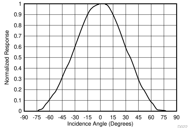
Figure 8-8. Angular Response of this FPCB Design Along the More-Restricted Rotational Axis
