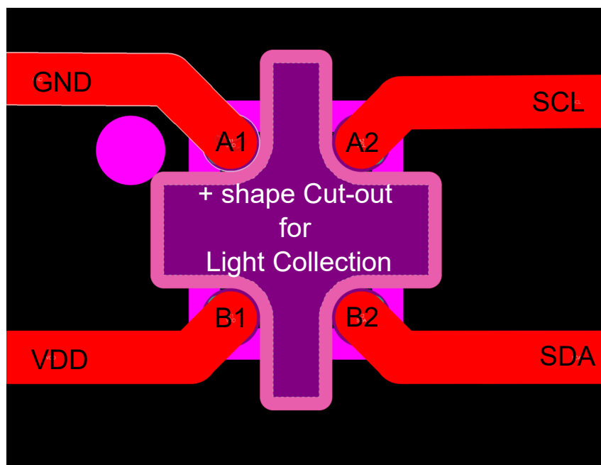
Figure 8-13. Layout Example for YMN Package With Plus-Shaped Cut Out
