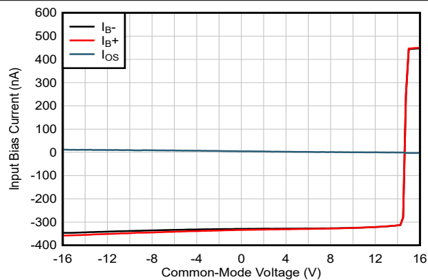
Figure 5-11. Input Bias Current and Offset Current vs Common-Mode Voltage
