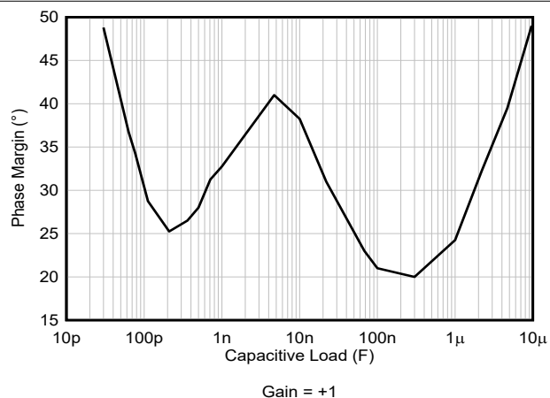
Figure 5-40. Phase Margin vs Capacitive Load
