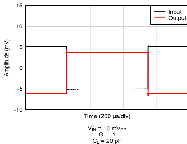
Figure 5-45. Small-Signal Step Response
