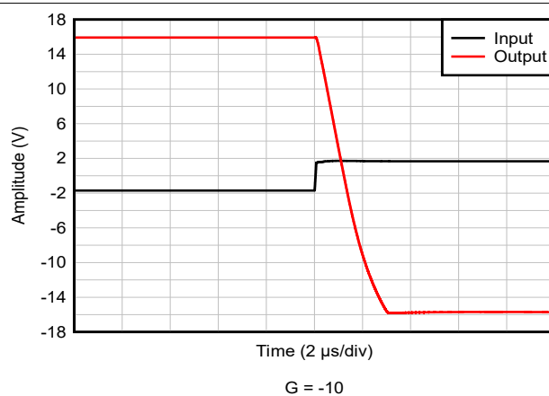
Figure 5-42. Positive Overload Recovery
