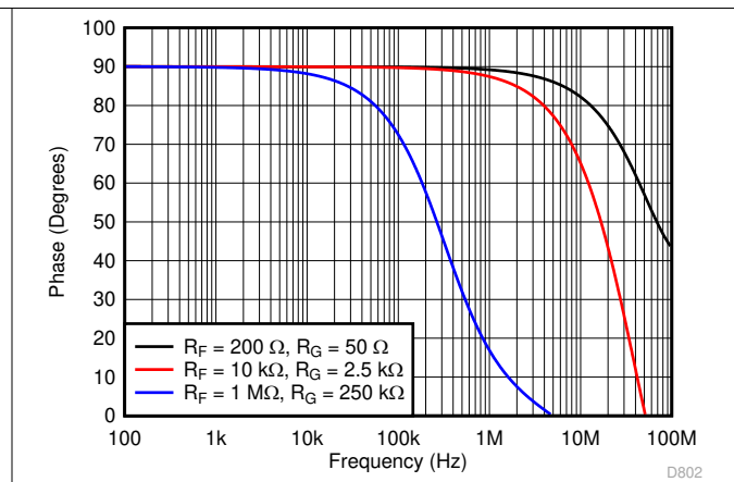
Figure 8-7. Loop-Gain Phase vs Frequency for Circuit of Figure 8-5
