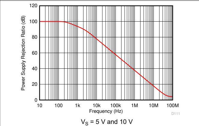
Figure 6-51. Power Supply Rejection Ratio vs Frequency
