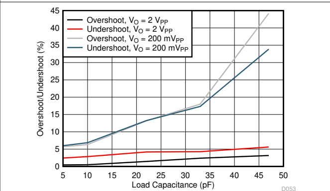
See Figure 8-1, gain = 1 V/V, R_F = 0\ \Omega
