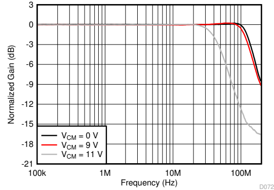
See Figure 8-1, V_O = 20\text{ mV}_{PP} , gain = 1\text{ V/V} , C_L = 4.7\text{ pF} , R_F = 0\ \Omega
