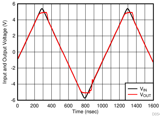
See Figure 8-1, gain = 1 V/V, R_F = 0\ \Omega
