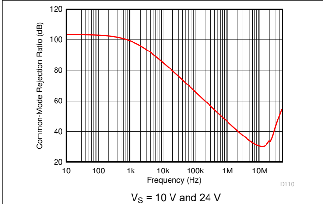
Figure 6-50. Common-Mode Rejection Ratio vs Frequency
