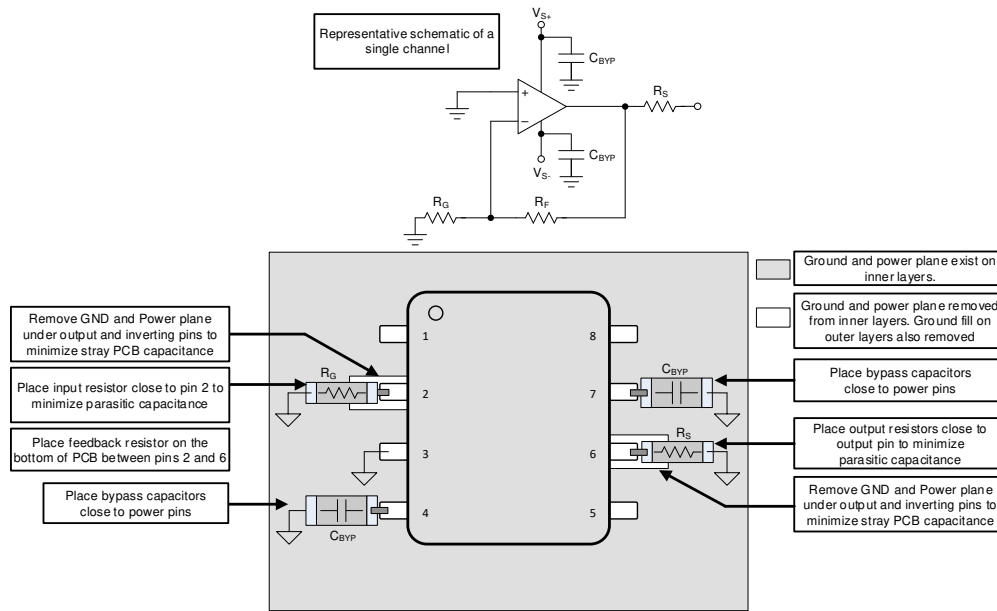
Figure 8-19. Layout Recommendation
