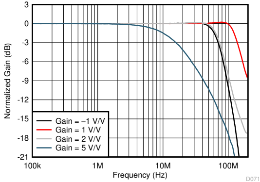
See Figure 8-1 and Figure 8-2, V_O = 20\text{ mV}_{PP}
