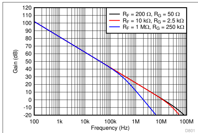
Figure 8-6. Loop-Gain vs Frequency for Circuit of Figure 8-5
