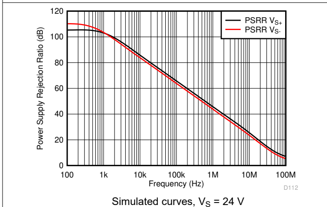
Figure 6-52. Power Supply Rejection Ratio vs Frequency
