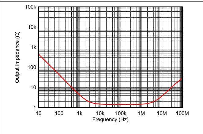
Figure 6-49. Open-Loop Output Impedance vs Frequency
