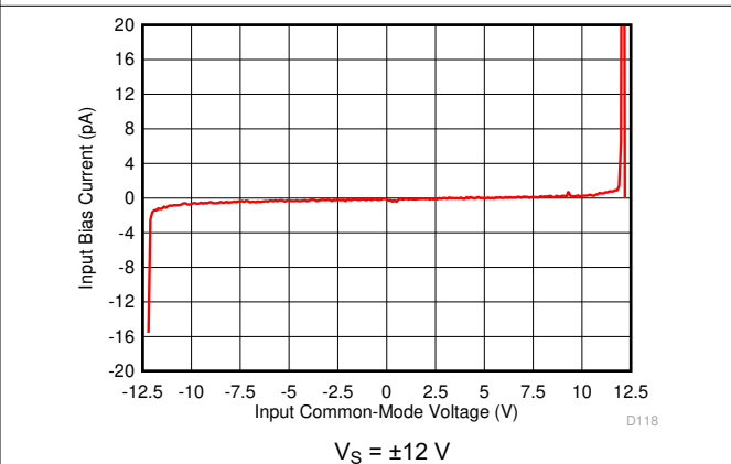
Figure 6-53. Input Bias Current vs Input Common-Mode Voltage
