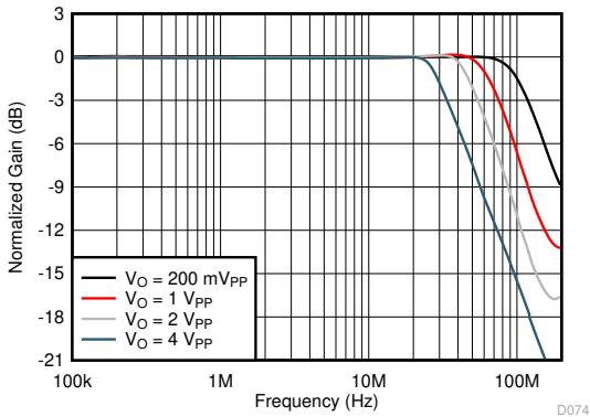
See Figure 8-1, gain = 1\text{ V/V} , R_F = 0\ \Omega
