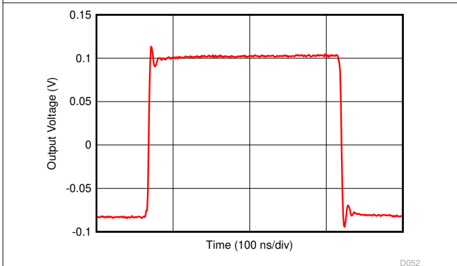
See Figure 8-1, gain = 1 V/V, R_F = 0\ \Omega , C_L = 10\text{ pF}
