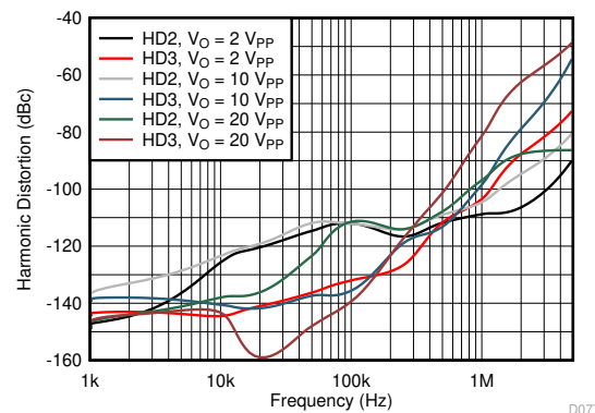
See Figure 8-2, gain = -1\text{ V/V}
