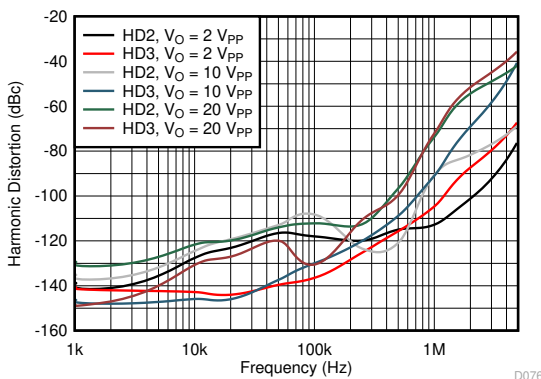
See Figure 8-1, gain = 2\text{ V/V}
