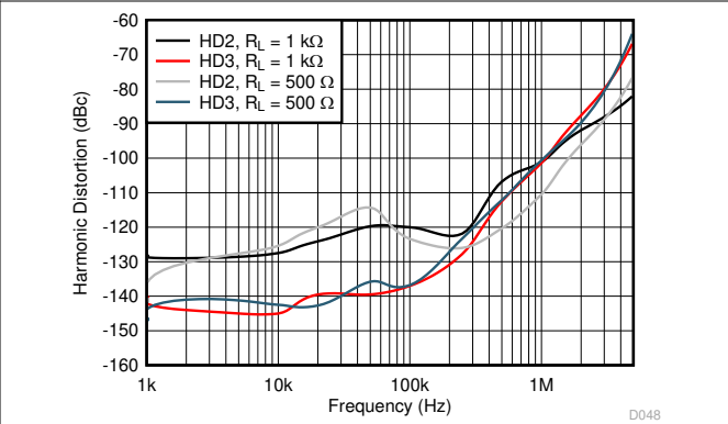
See Figure 8-1, gain = 2 V/V
