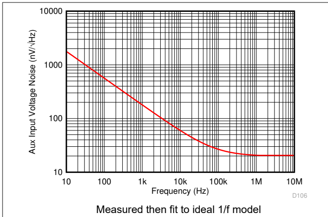
Figure 6-48. Auxiliary Input Stage Voltage Noise Density vs Frequency
