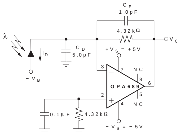
Figure 35. Transimpedance Amplifier
