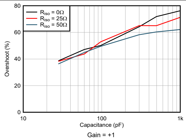
Figure 5-30. Small-Signal Overshoot vs Capacitive Load
