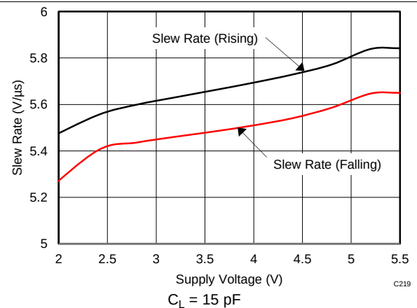
Figure 34. Slew Rate vs Supply Voltage
