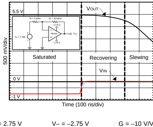
Figure 27. Positive Overload Recovery
