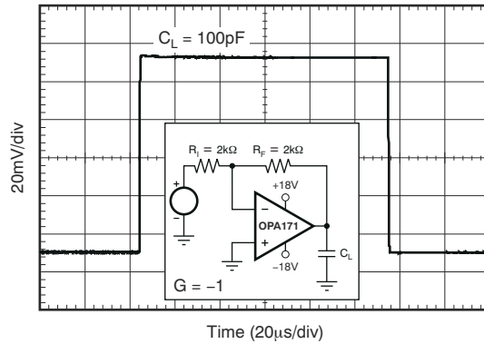
Figure 5-29. Small-Signal Step Response (100 mV)
