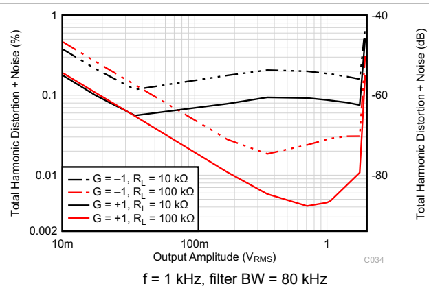
Figure 5-24. THD+N vs Output Amplitude
