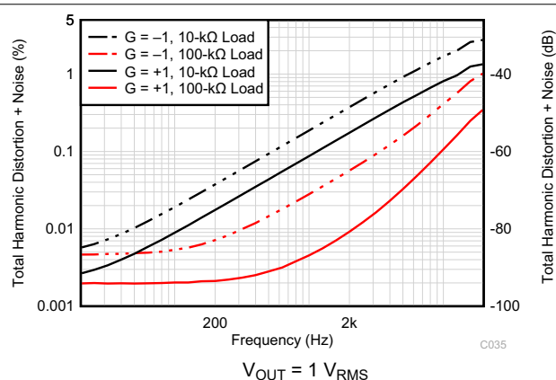
Figure 5-23. THD+N Ratio vs Frequency
