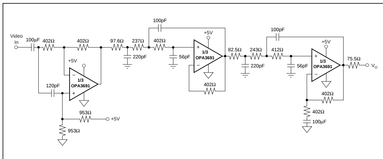
FIGURE 5. Filter Schematic.
