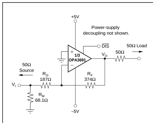
FIGURE 11. Inverting Gain of -2 with Impedance Matching.
