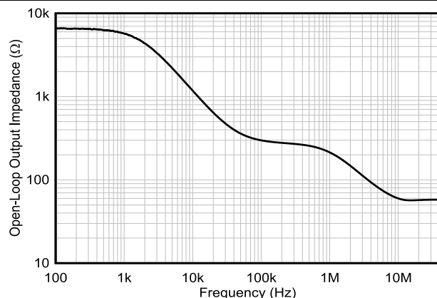
Figure 5-35. Open-Loop Output Impedance vs Frequency
