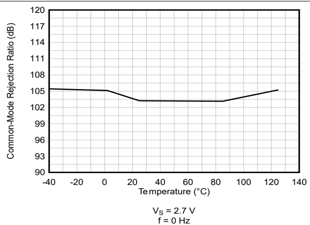
Figure 5-24. CMRR vs Temperature
