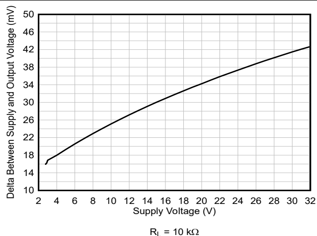
Figure 5-36. Output Swing vs Supply Voltage, Positive Swing
