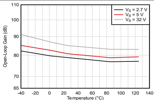
Figure 5-34. Open-Loop Voltage Gain vs Temperature (dB)
