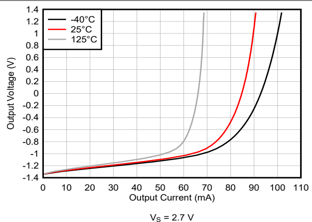
Figure 5-20. Output Voltage Swing vs Output Current (Sinking)
