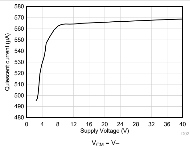
Figure 6-23. Quiescent Current vs Supply Voltage V_{CM} = V_-
