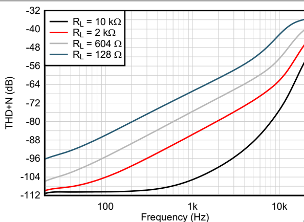
Figure 6-21. THD+N Ratio vs Frequency BW = 80 kHz, V_{OUT} = 1\text{ V}_{RMS}
