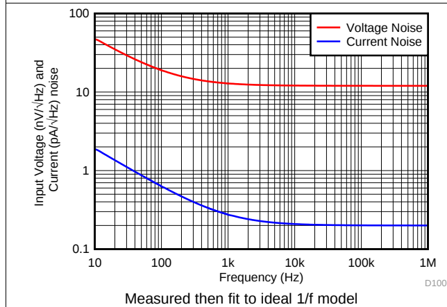
Figure 31. Input Noise Density vs Frequency
