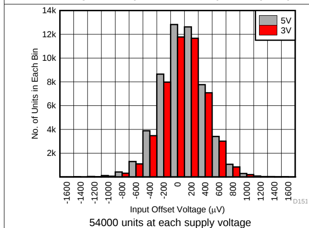
Figure 33. Input Offset Voltage Distribution
