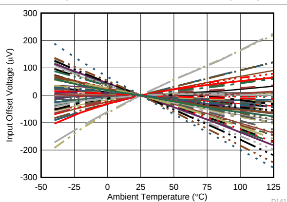
Figure 34. Input Offset Voltage vs Ambient Temperature
