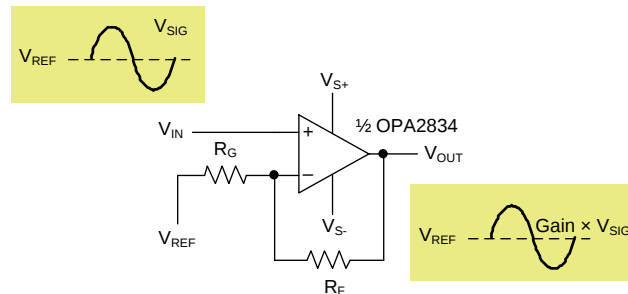
Figure 45. Noninverting Amplifier
