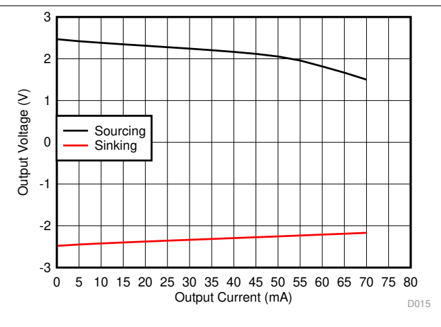
Figure 41. Output Voltage Range vs Output Current
