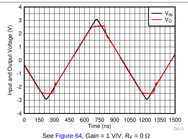
Figure 39. Input Overdrive Recovery
