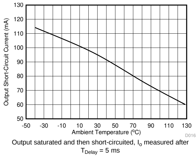
Figure 42. Output Short-Circuit Current vs Ambient Temperature
