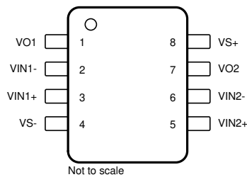
Pin Functions
