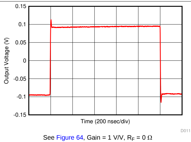
Figure 37. Small-Signal Transient Response
