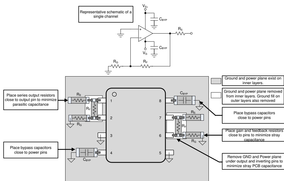
Figure 79. Layout Recommendation
