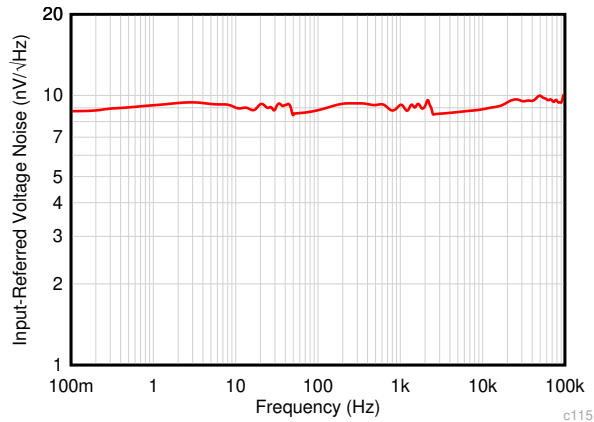
Figure 6-15. Input Voltage Noise Spectral Density vs Frequency
