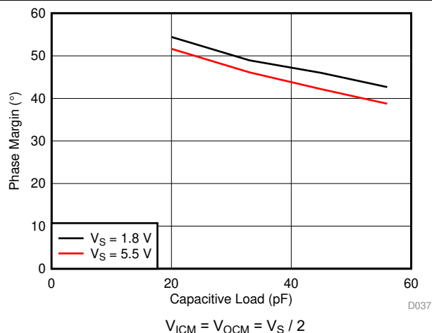
Figure 7-38. Phase Margin vs Capacitive Load
