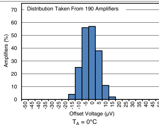
Figure 4. Offset Voltage Production Distribution at 0^\circ\text{C}
