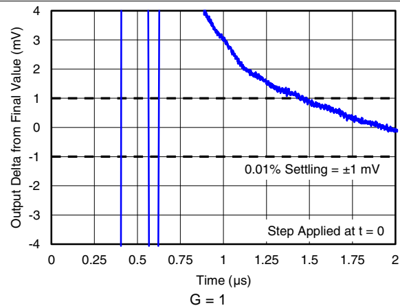
Figure 38. Settling Time (10-V Positive Step)
