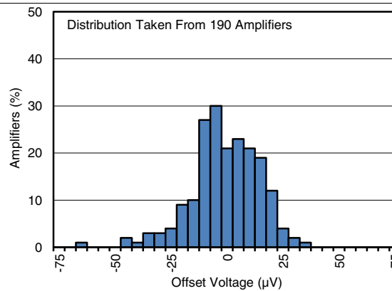
Figure 2. Offset Voltage Production Distribution at 125^\circ\text{C}
