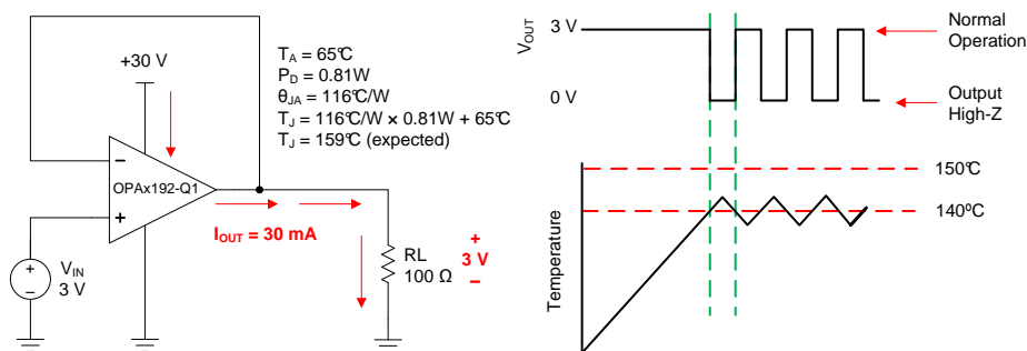
Figure 54. Thermal Protection
