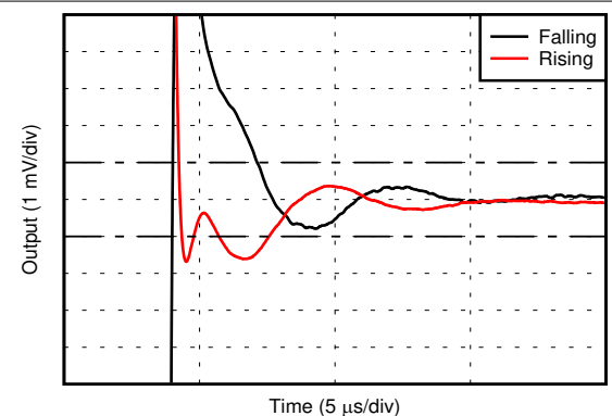
Figure 6-33. Large-Signal Step Response
