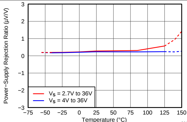
Figure 12. PSRR vs Temperature
